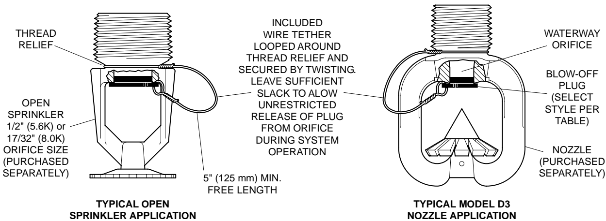
FIGURE 1 BLOW-OFF PLUGS
