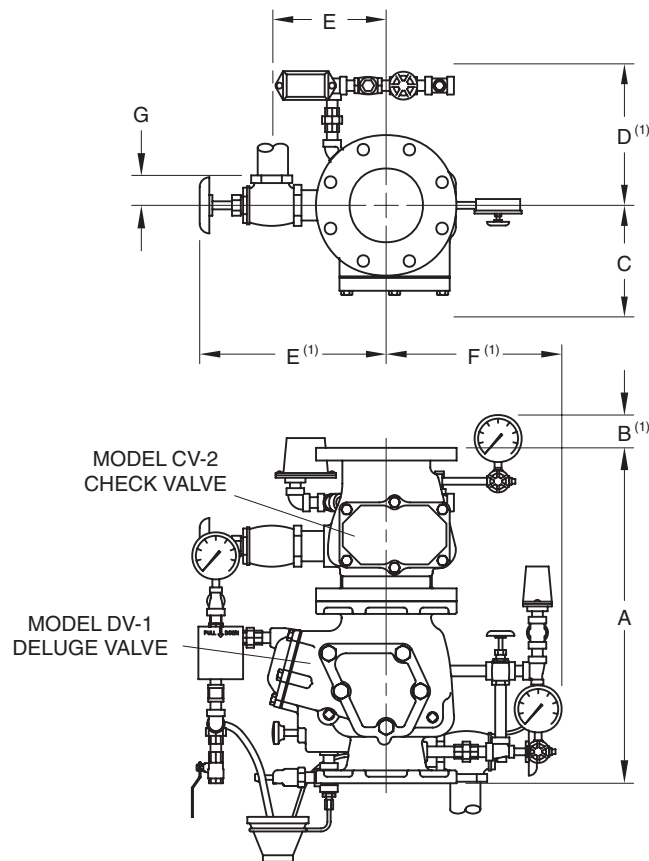
FIGURE 1 4 and 6 INCH (DN100 and DN150) SUPERVISED SINGLE INTERLOCK PREACTION SYSTEM RISER ARRANGEMENT
